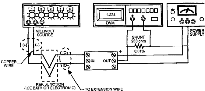
Typical Test Connection
